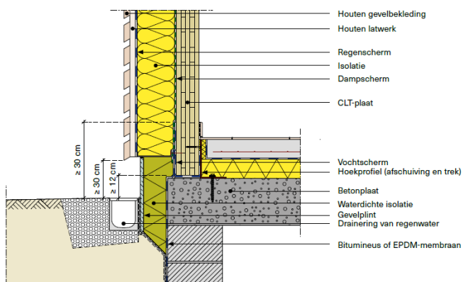
Figuur 36: Drainage
